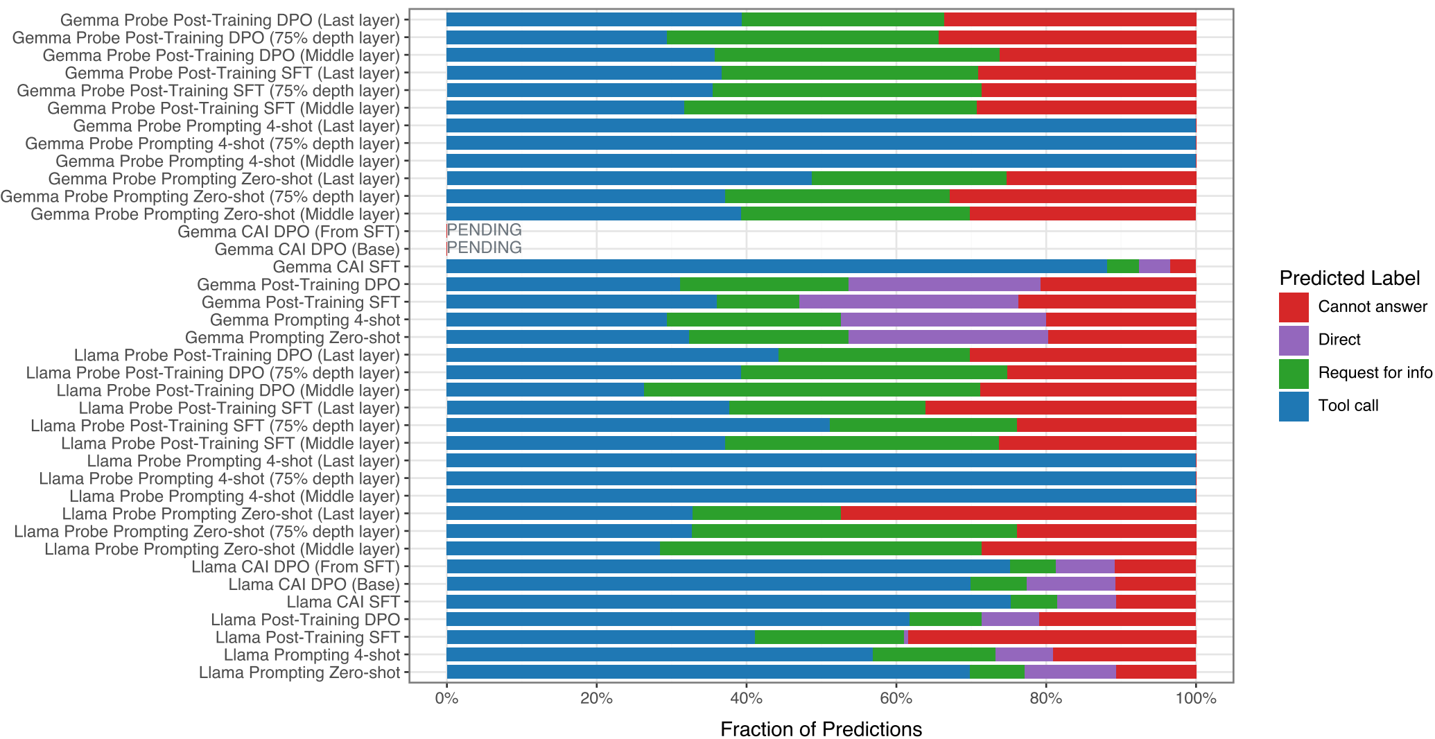
When2Call (hmm): Prompting + Post-Training + CAI + Probe - Normalized Prediction Mix by Run
