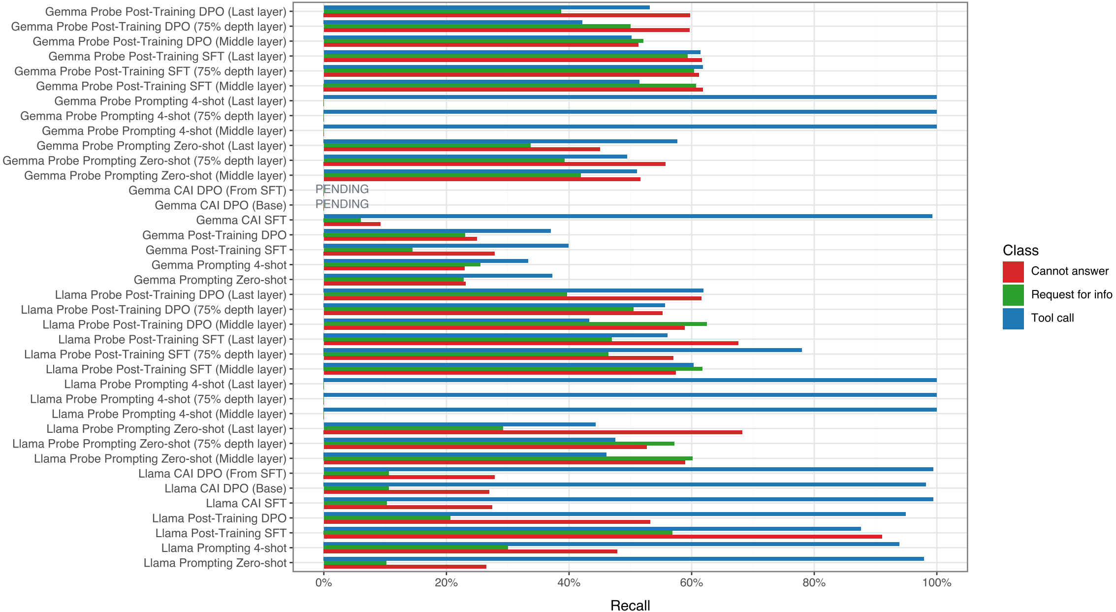
When2Call (hmm): Prompting + Post-Training + CAI + Probe - Per-Class Recall by Run (Normalized)
