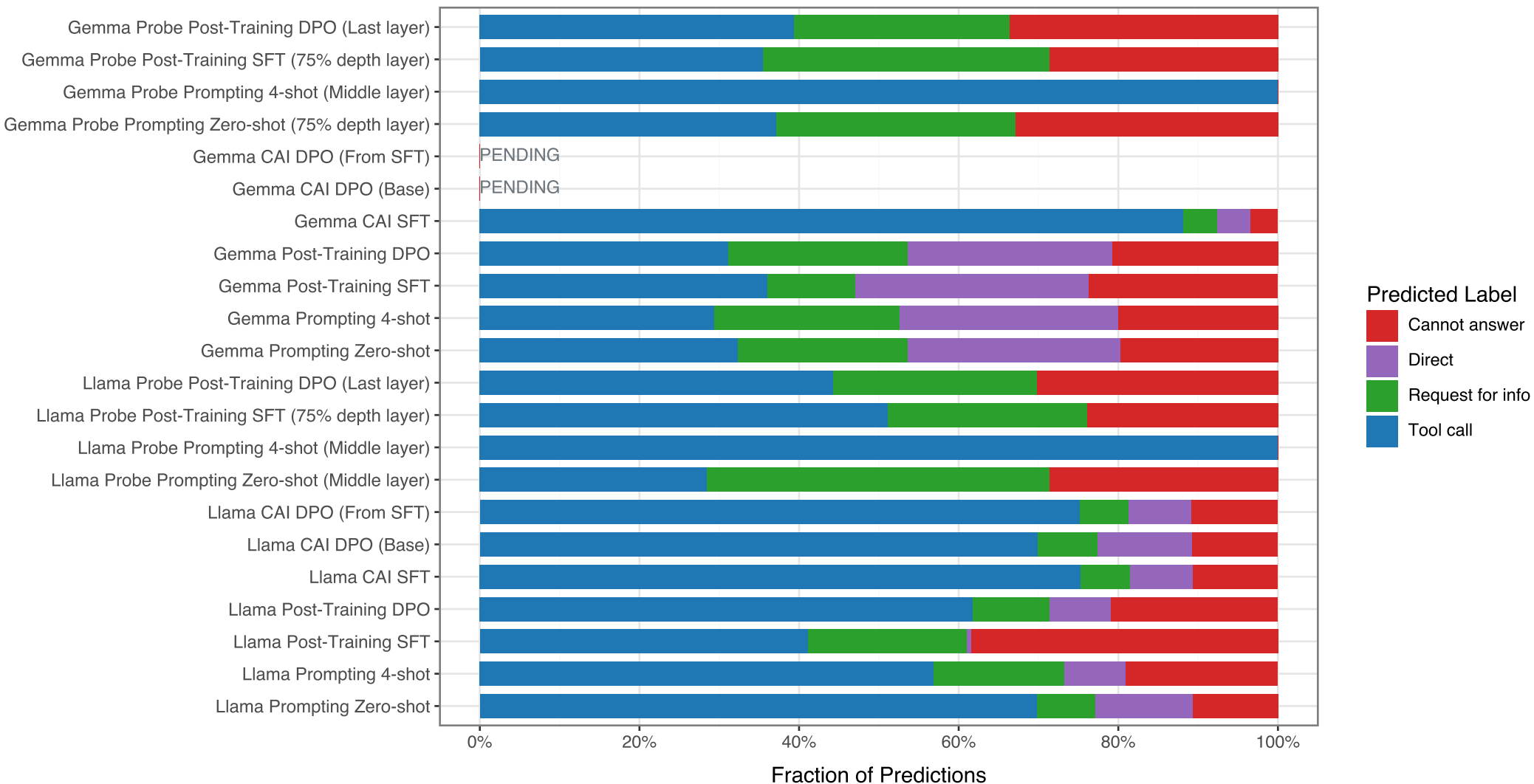
Prediction Mix on When2Call (All Runs)
