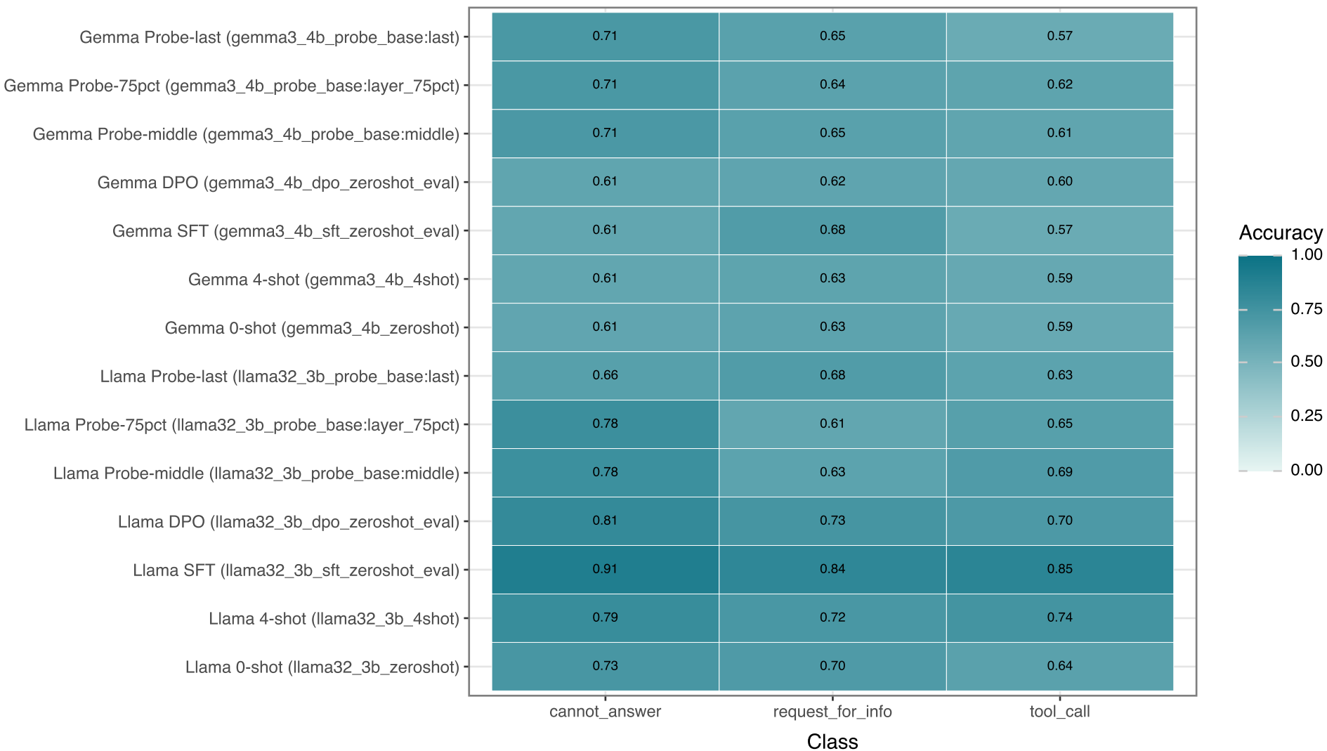
Per-Class Accuracy (One-vs-Rest)
