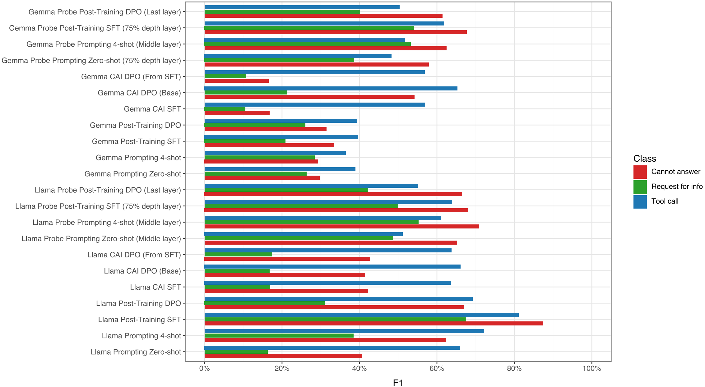
Per-Class F1 on When2Call (All Runs)
