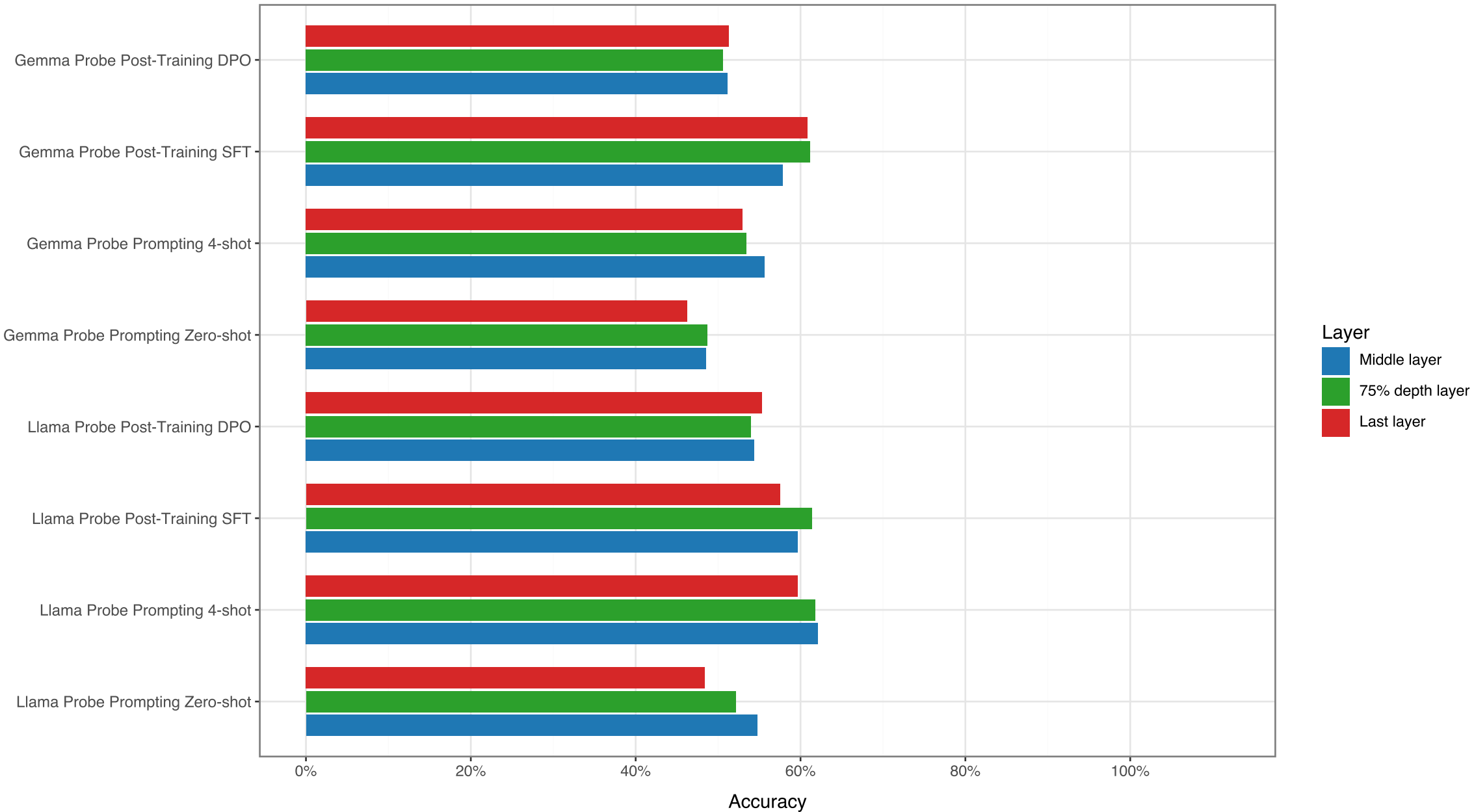
Probe Layer Accuracy on When2Call
