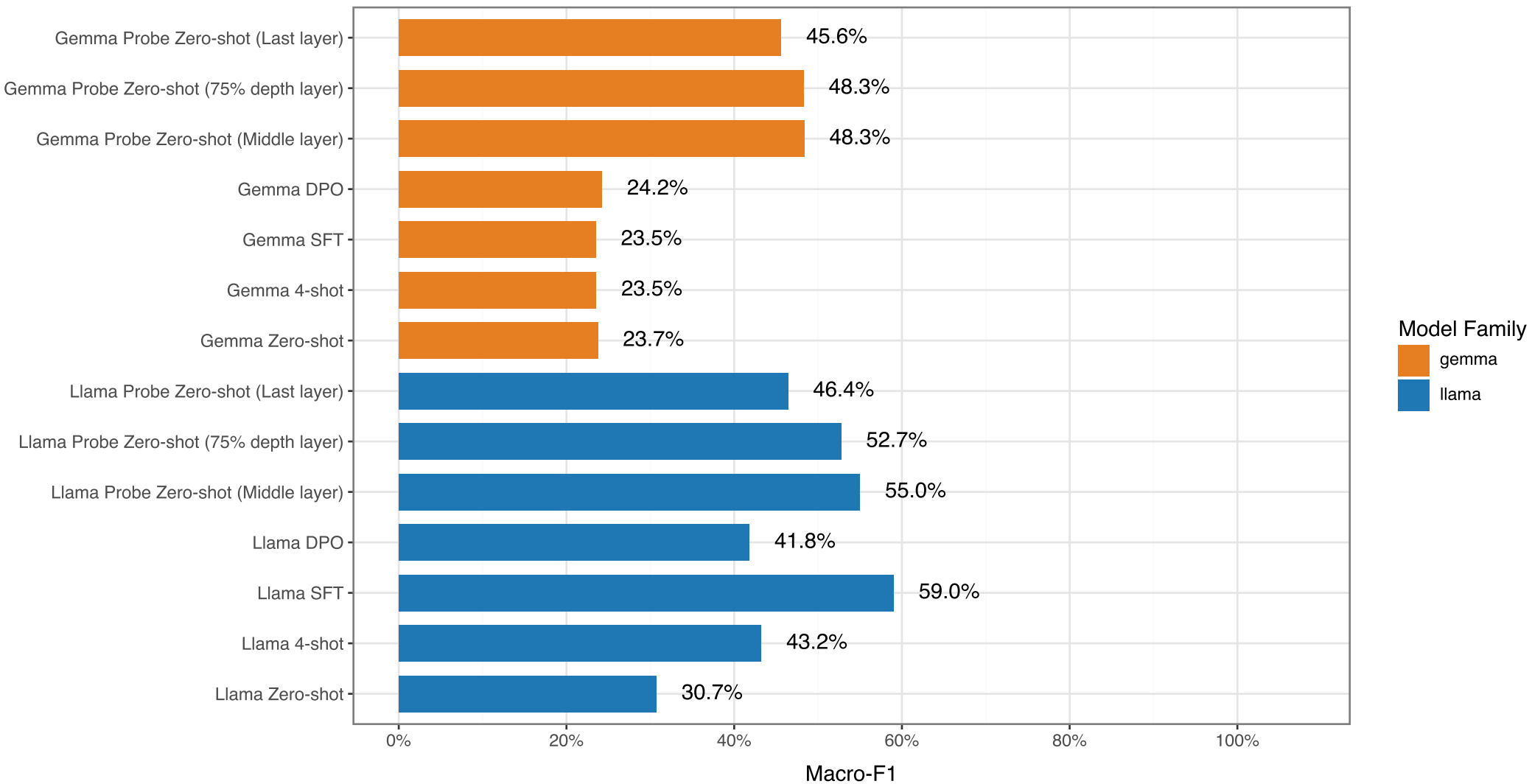
Normalized Macro-F1 by Run
