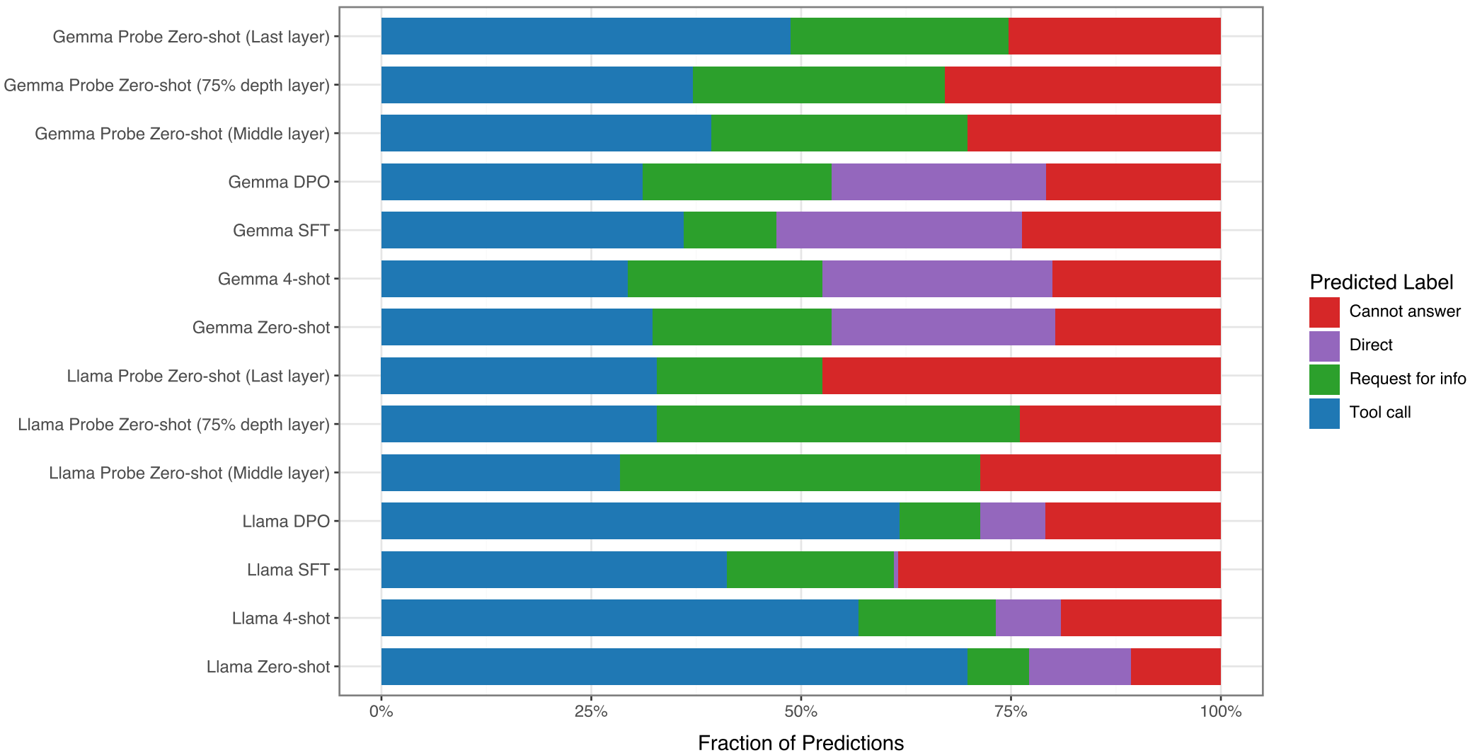
Normalized Prediction Mix by Run
