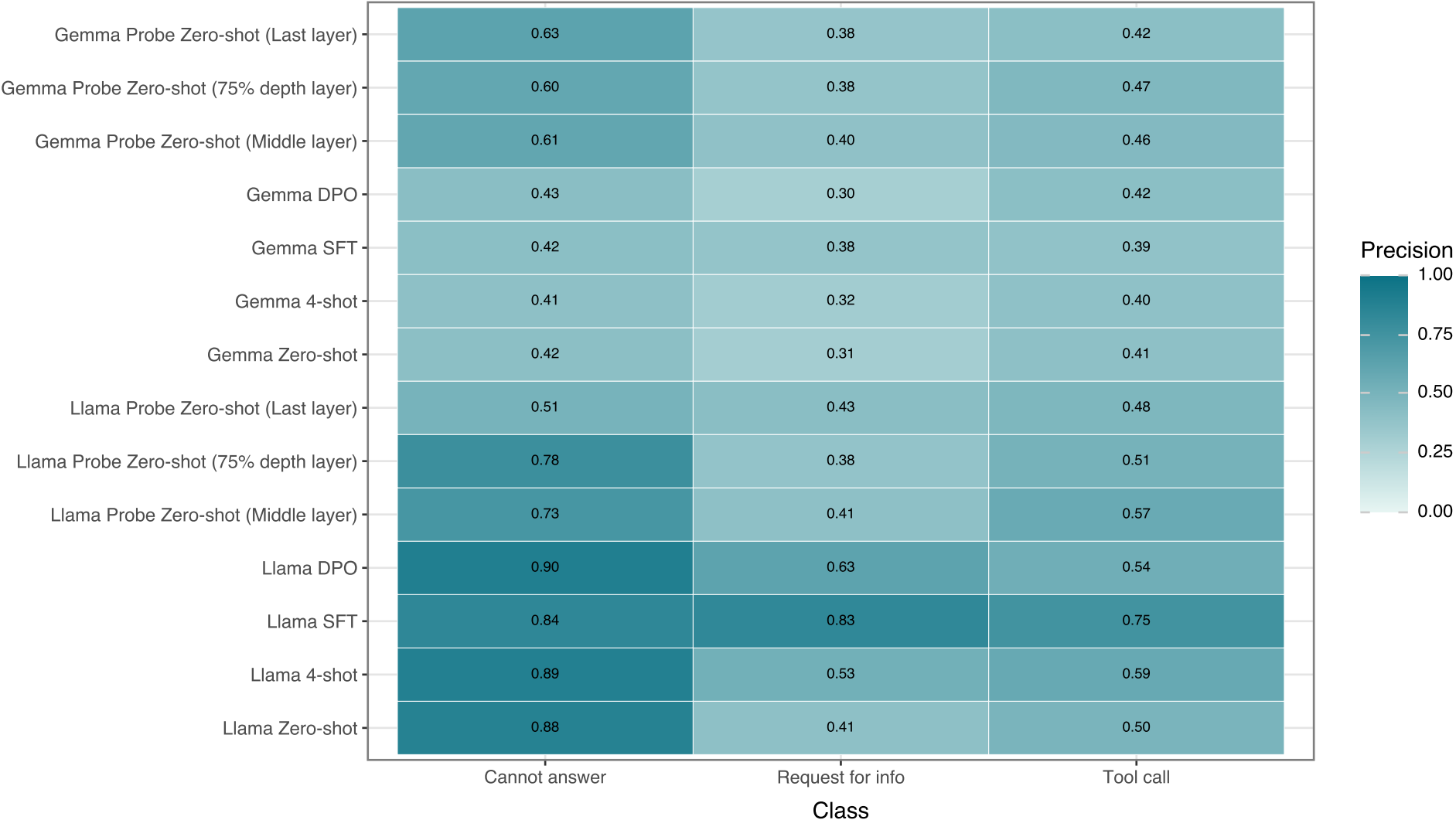
Per-Class Precision
