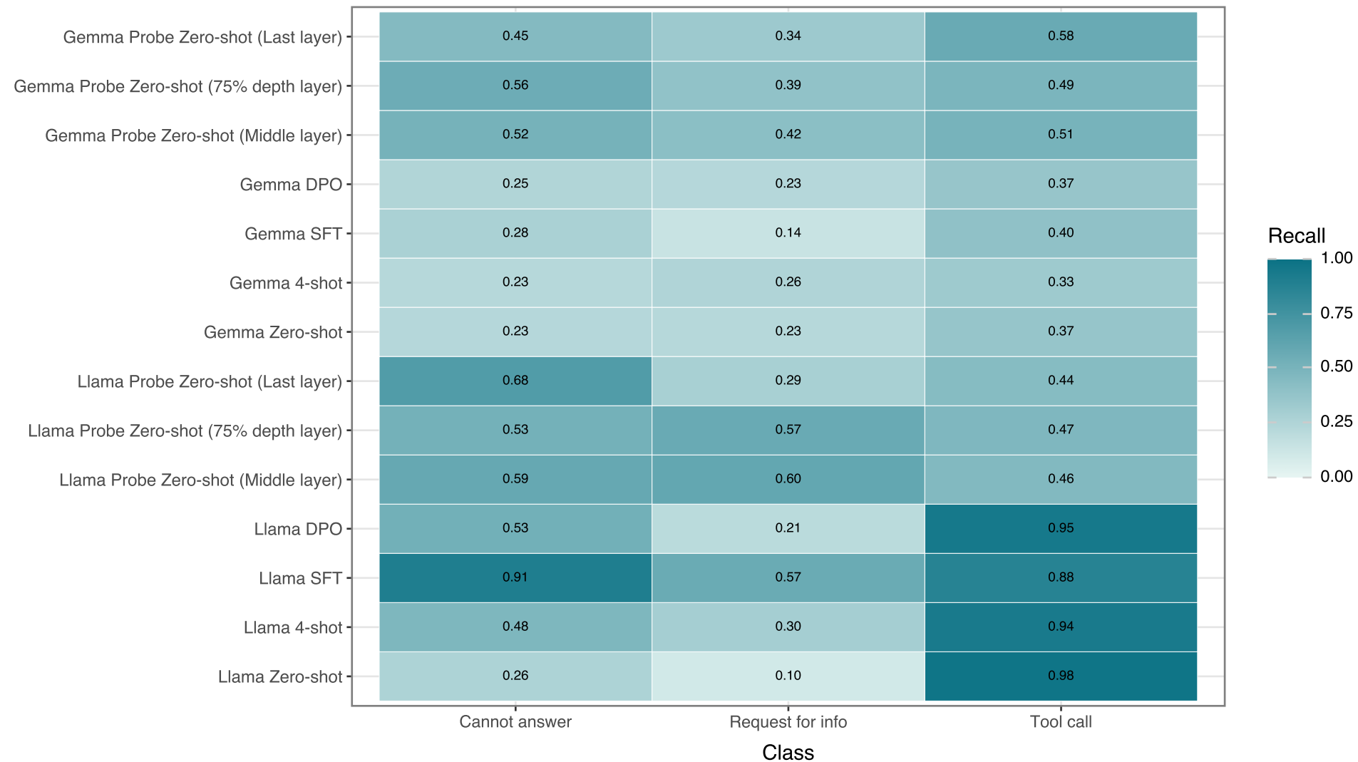
Per-Class Recall
