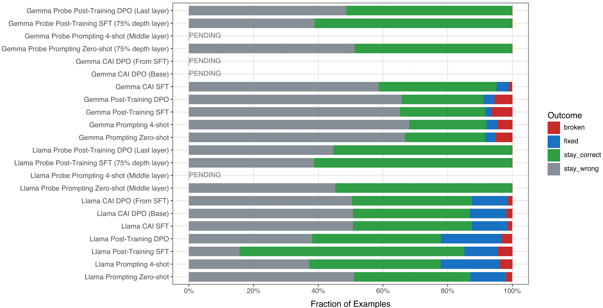
Normalization Outcome Breakdown on When2Call (All Runs)
