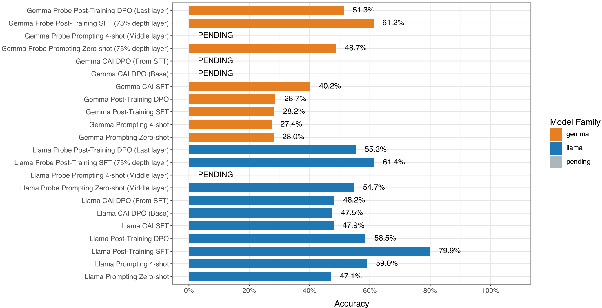
Accuracy on When2Call (All Runs)
