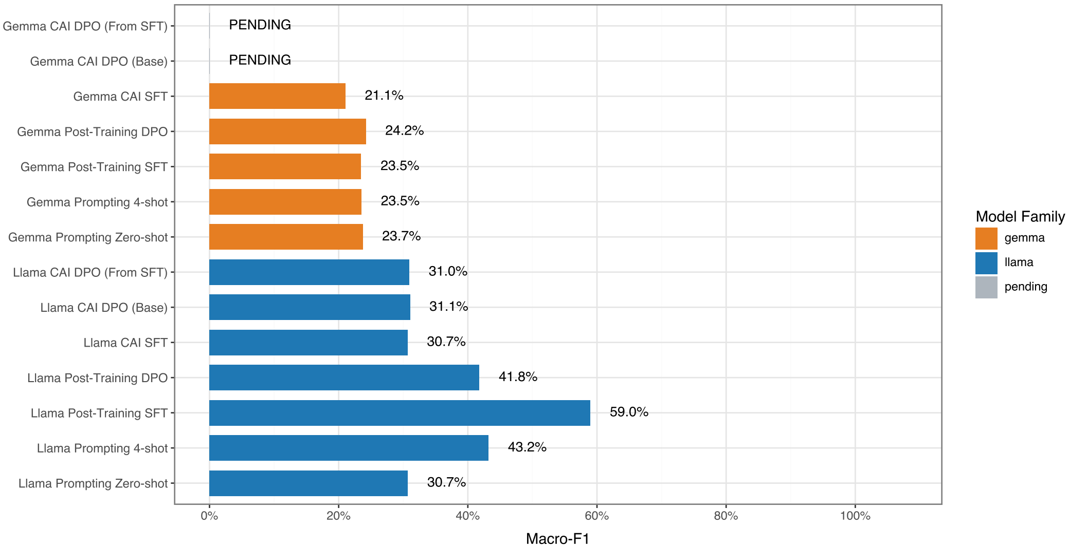
Macro-F1 on When2Call (No Probe)
