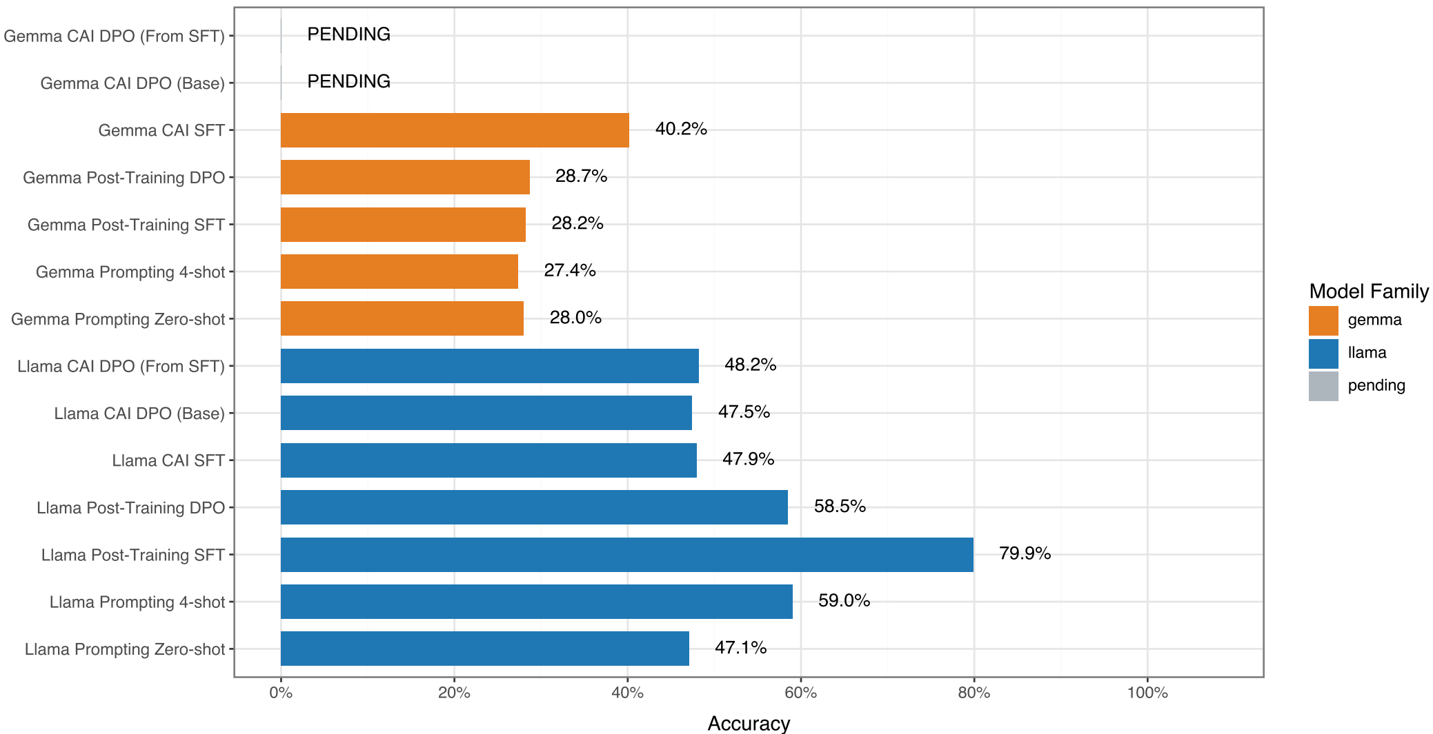
Normalized Accuracy on When2Call (No Probe)
