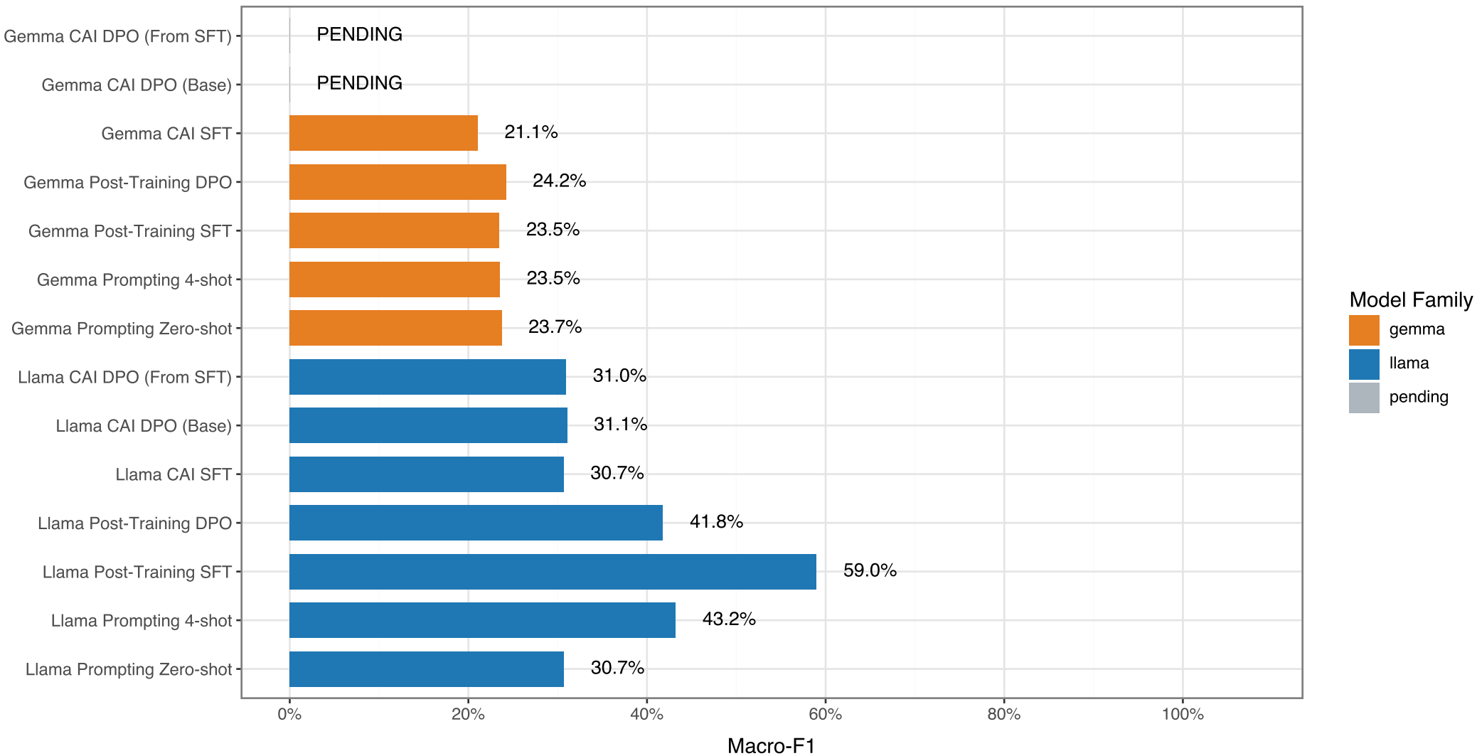
Normalized Macro-F1 on When2Call (No Probe)
