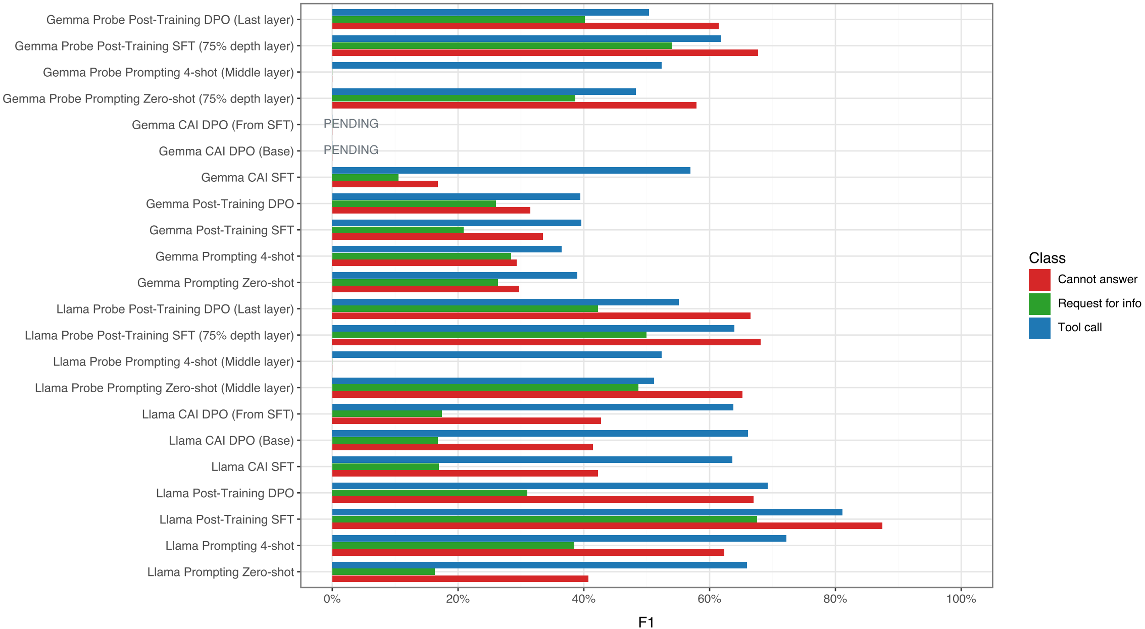
Per-Class F1 (Normalized) on When2Call (All Runs)
