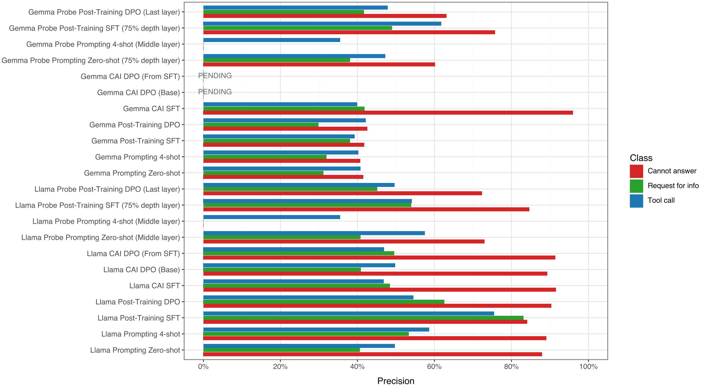
Per-Class Precision (Normalized) on When2Call (All Runs)
