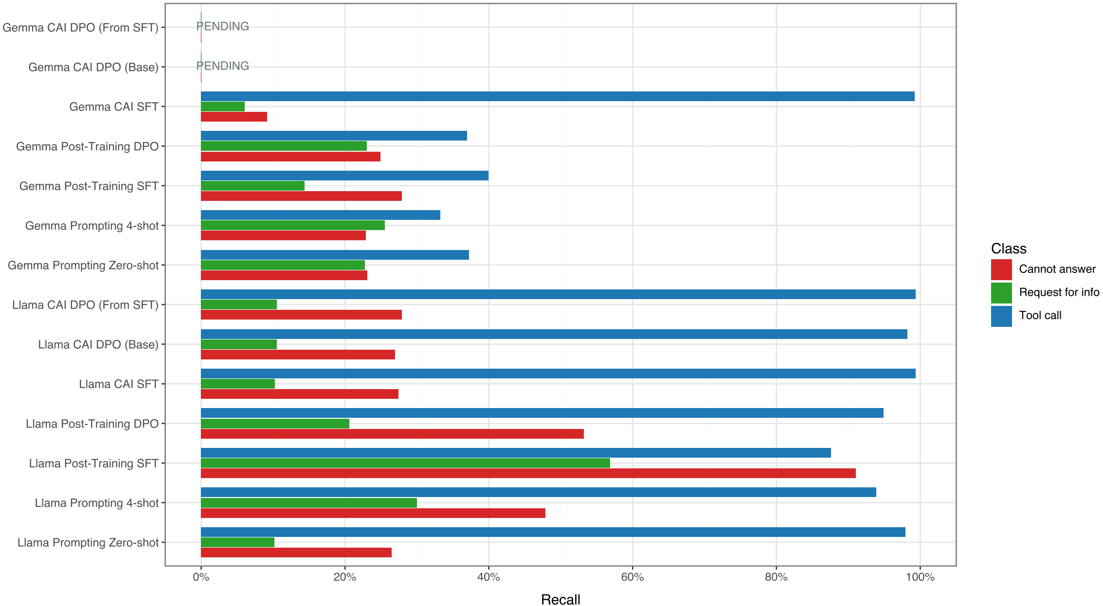
Per-Class Recall (Normalized) on When2Call (No Probe)
