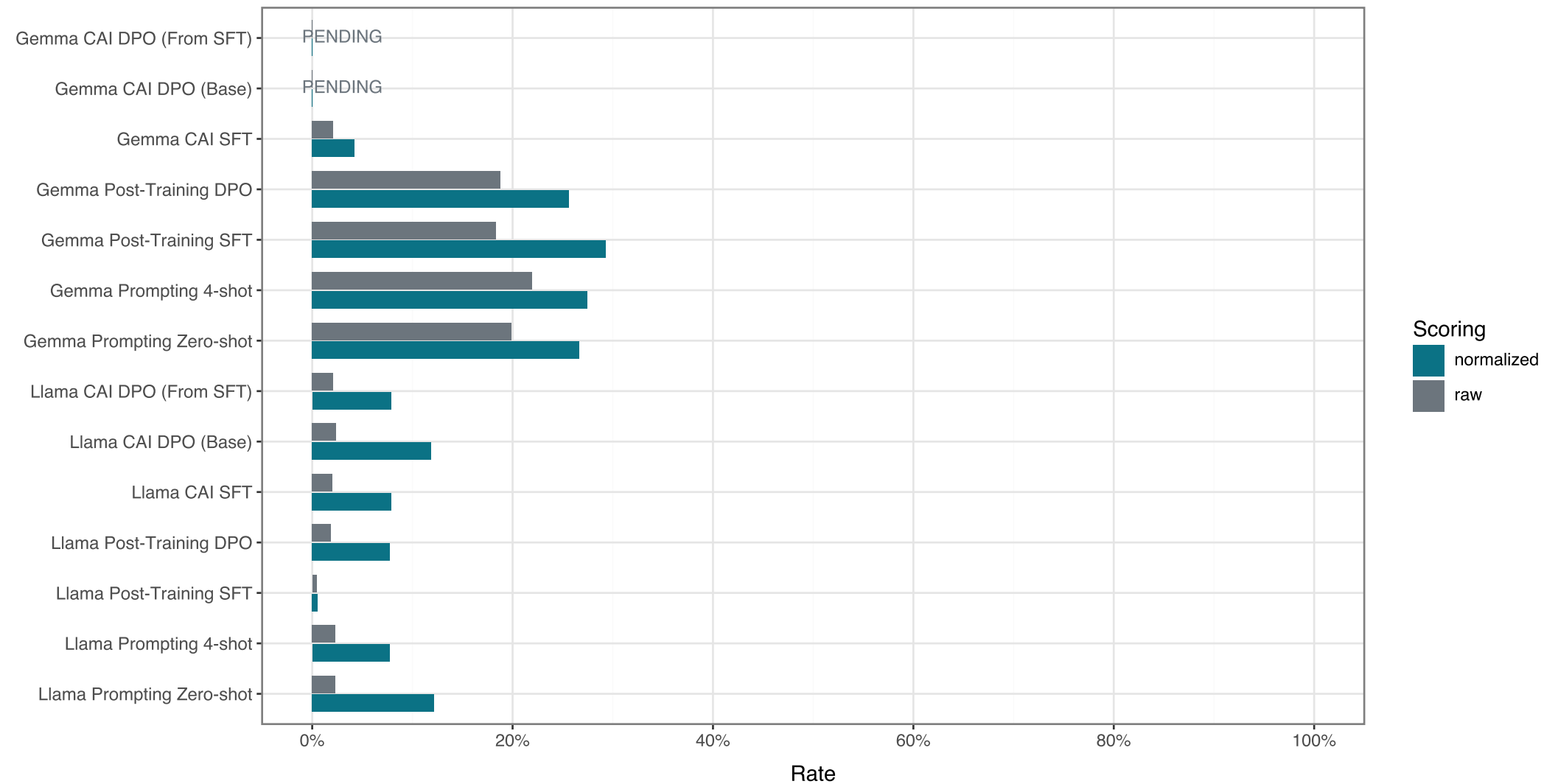
Unsupported 'direct' Prediction Rate on When2Call (No Probe)
