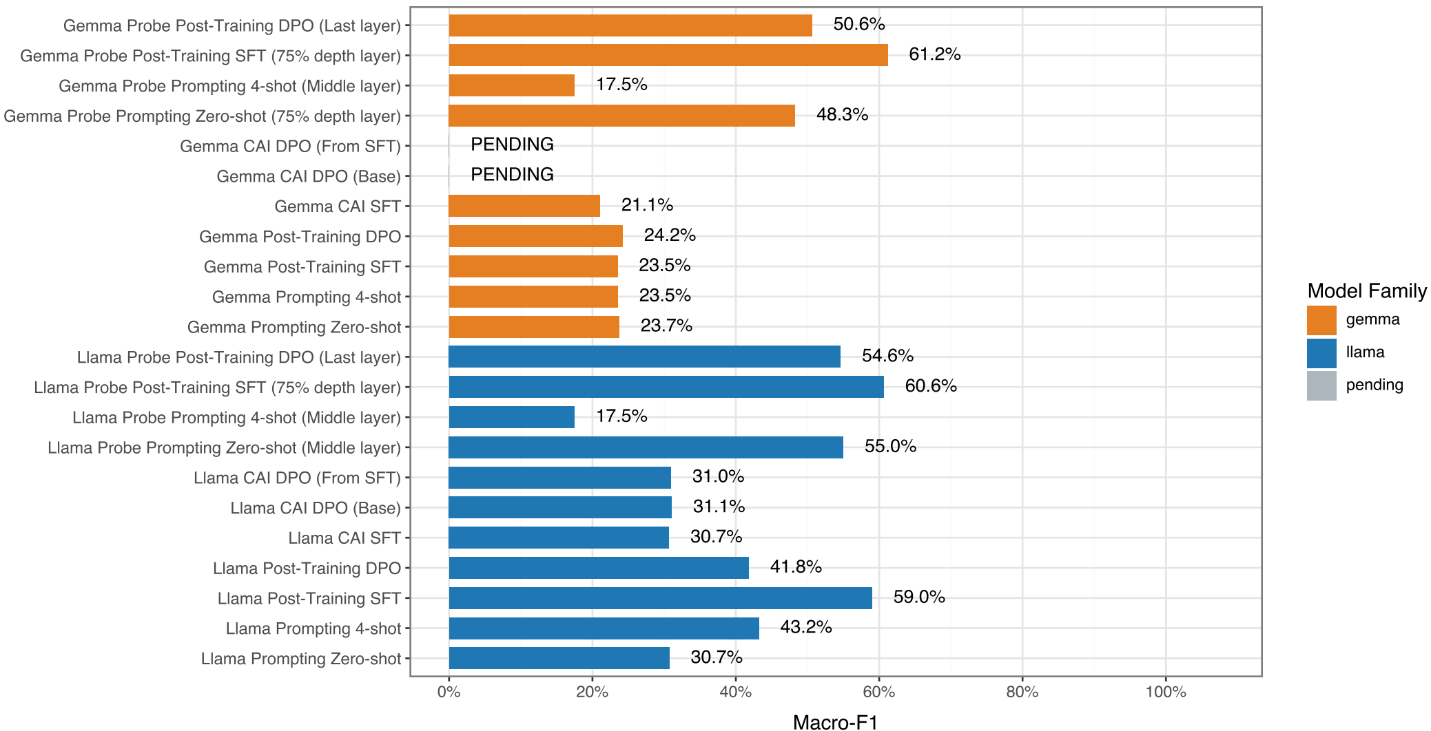
Macro-F1 on When2Call (All Runs)
