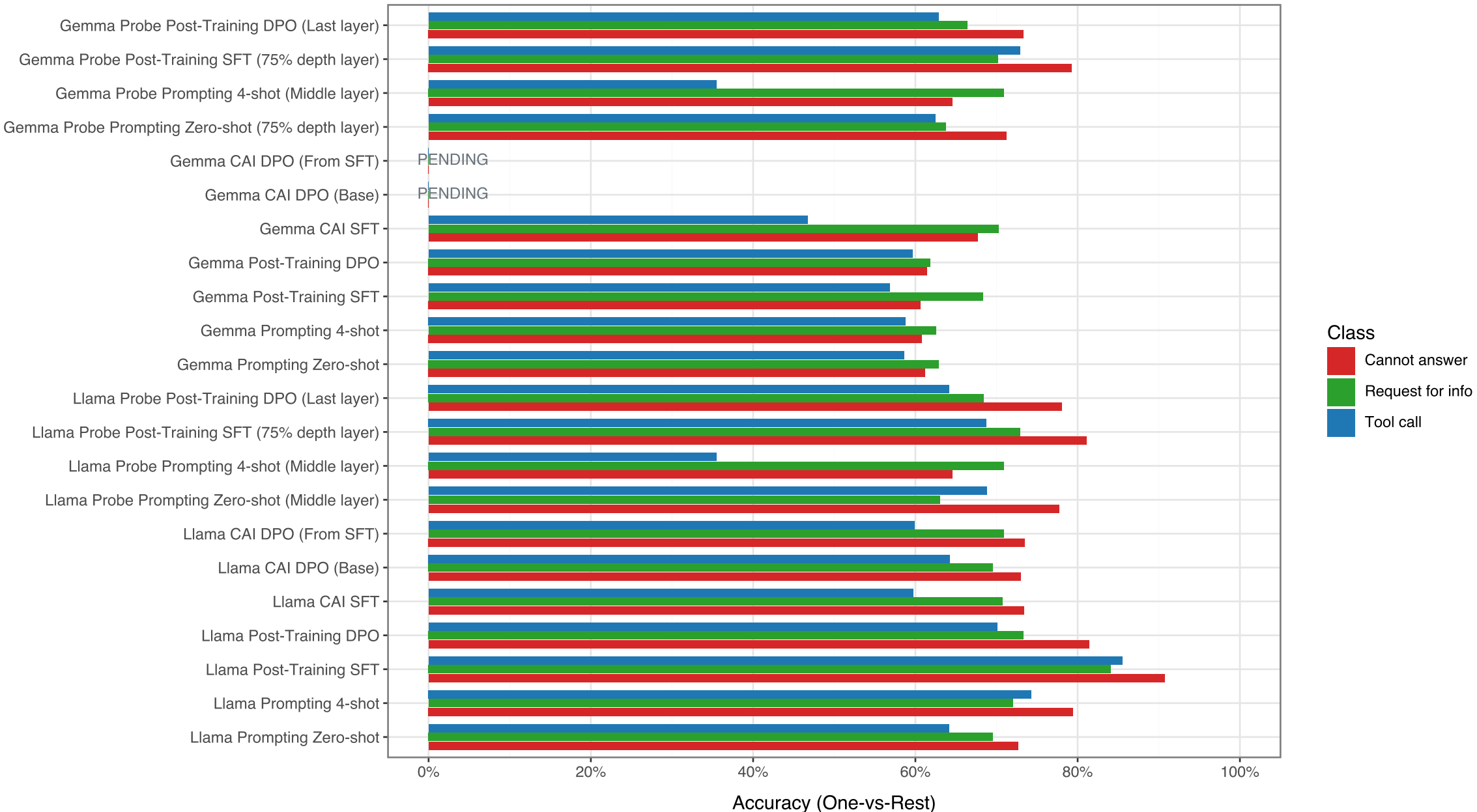
Per-Class Accuracy on When2Call (All Runs)
