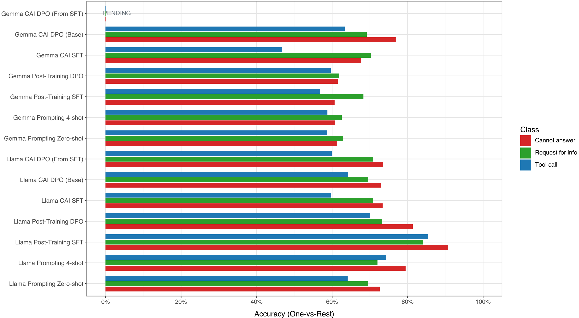
Per-Class Accuracy on When2Call (No Probe)
