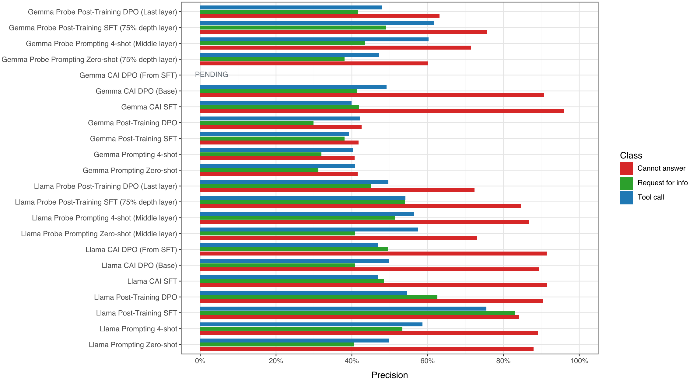
Per-Class Precision on When2Call (All Runs)
