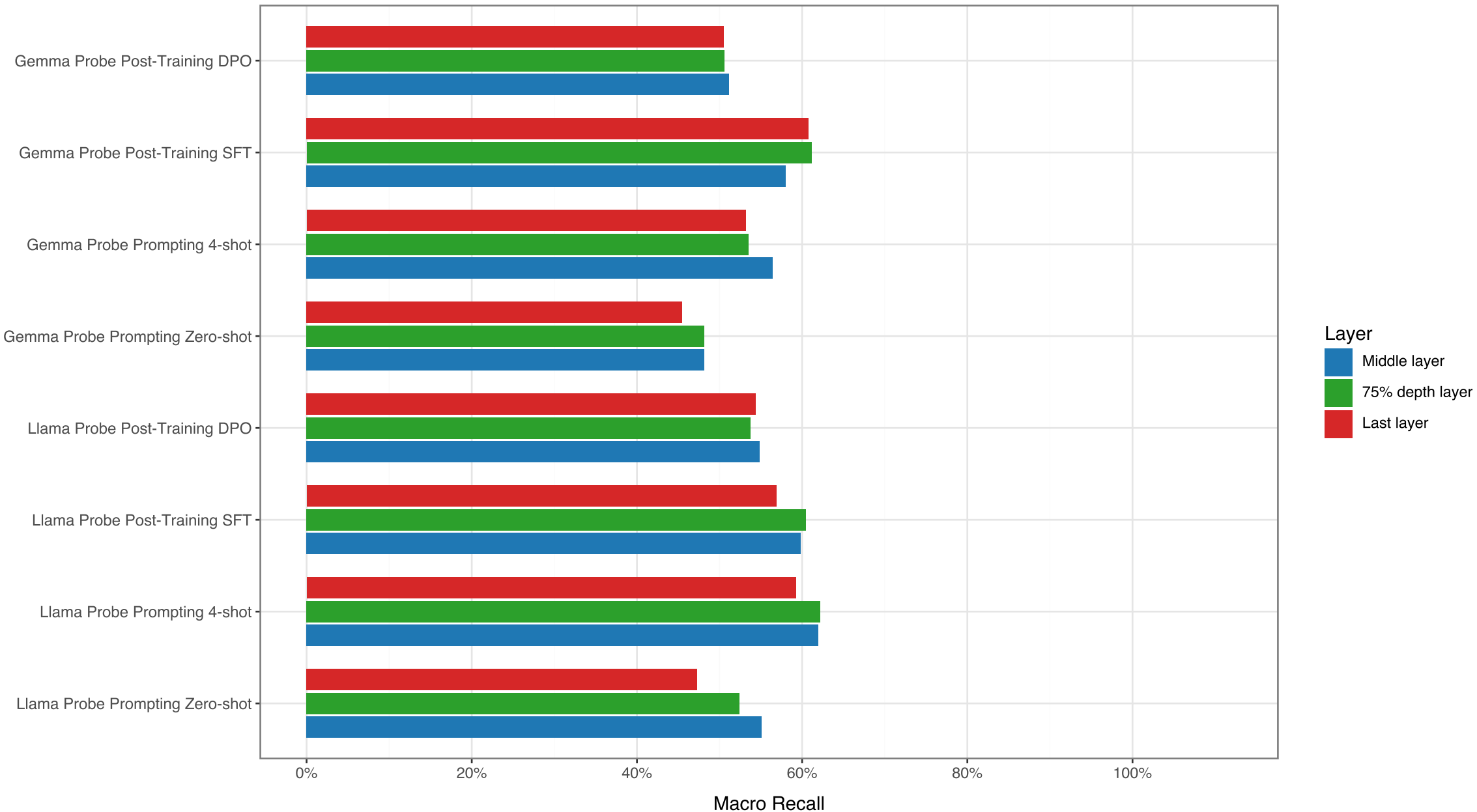
Probe Layer Macro Recall on When2Call
