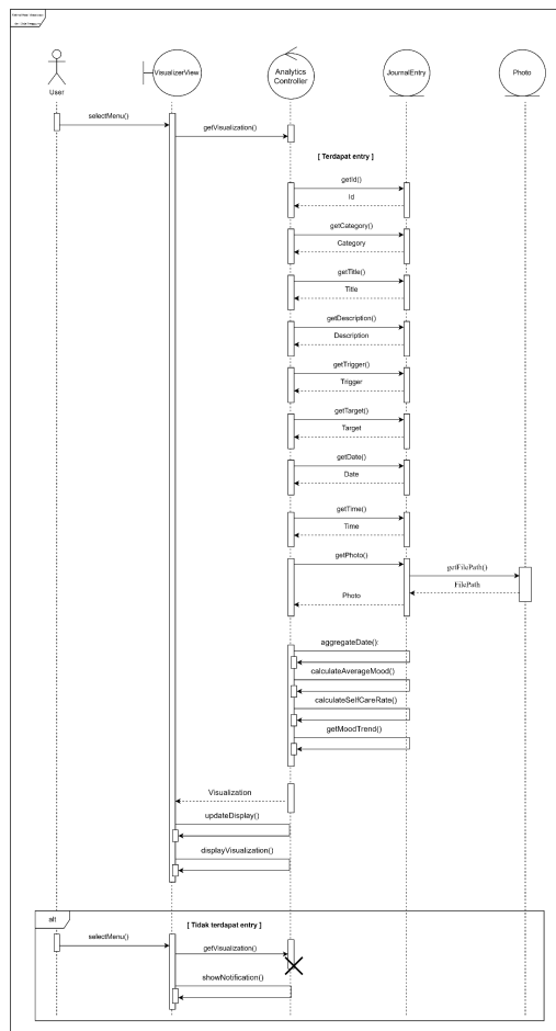
Gambar 3.2. Sequence Diagram UC02
