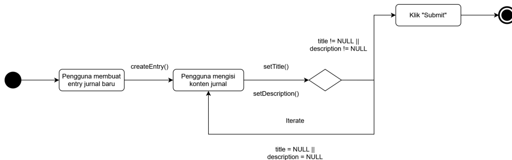
Gambar 3.8 Diagram Statechart
