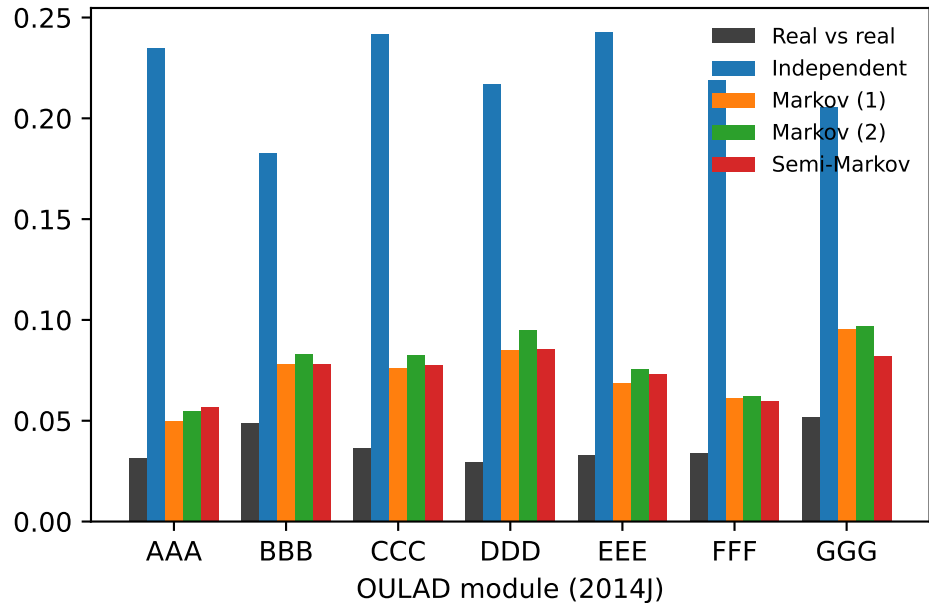
Bigram TVD (lower is better)
