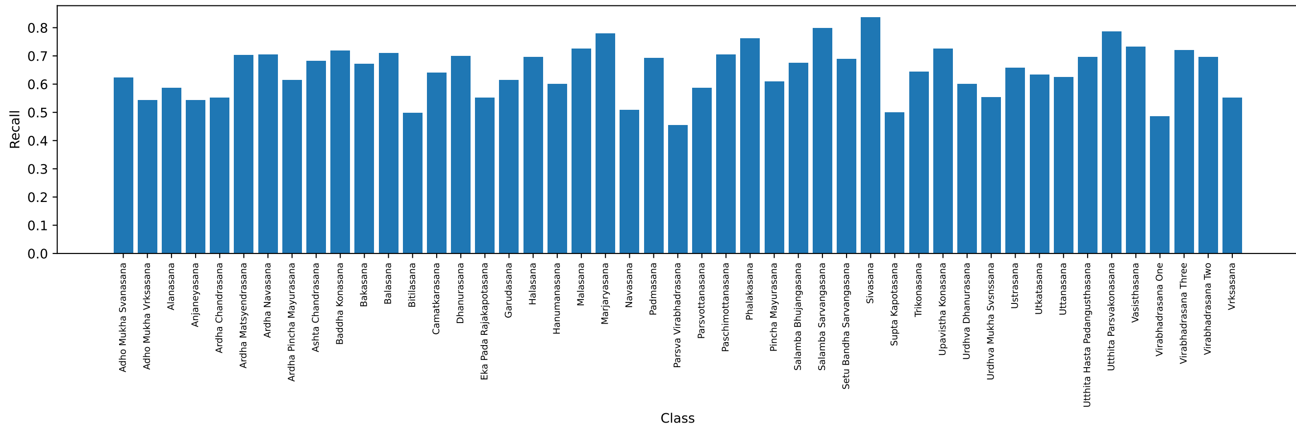
Per-class Recall
