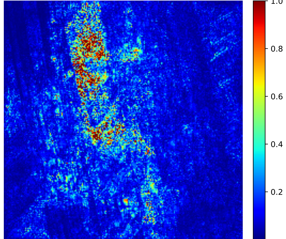
SHAP Heatmap
