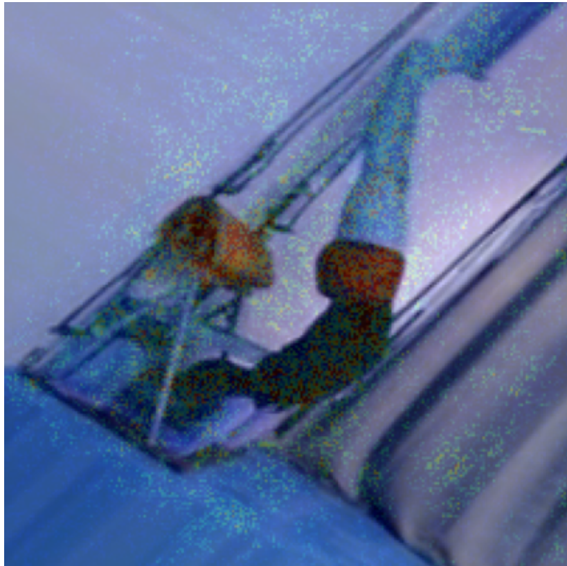
SHAP Overlay
