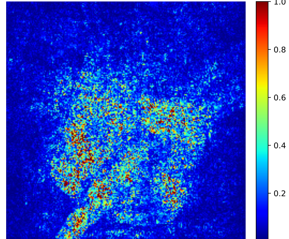
SHAP Heatmap
