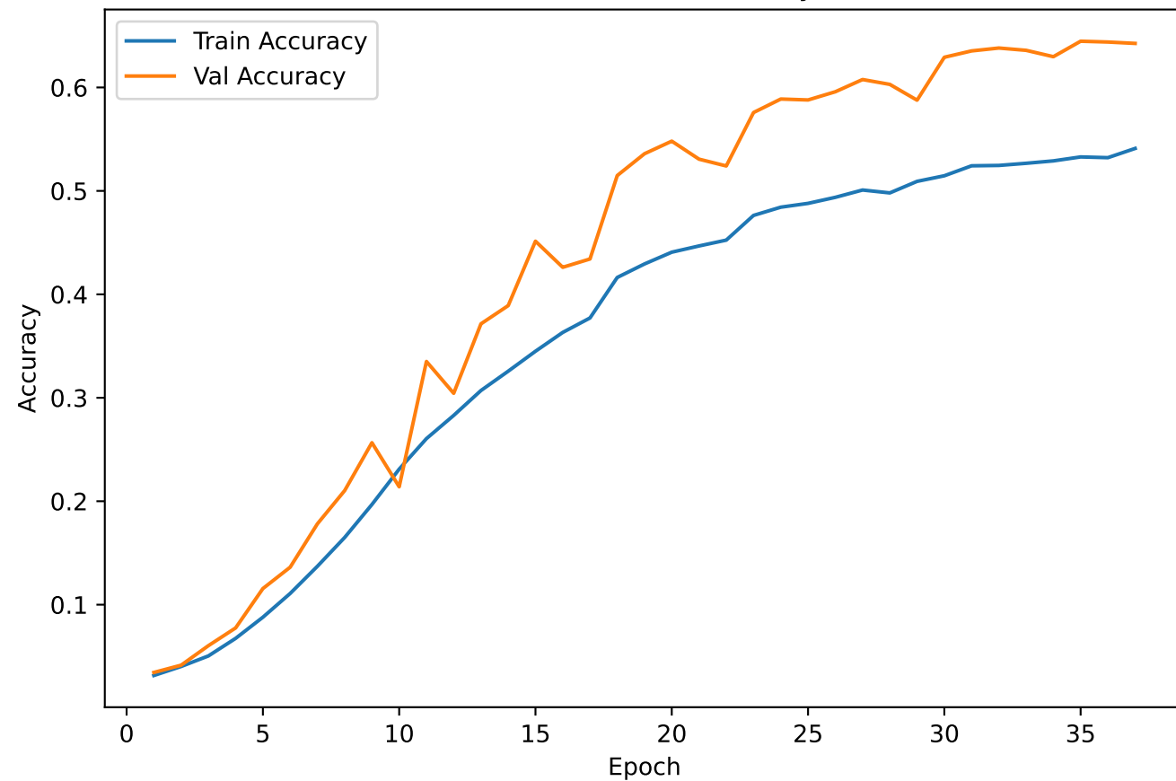
Custom CNN - Accuracy
