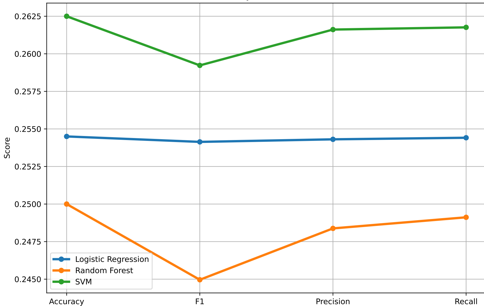
RQ5 Sensitivity to Evaluation Metrics
