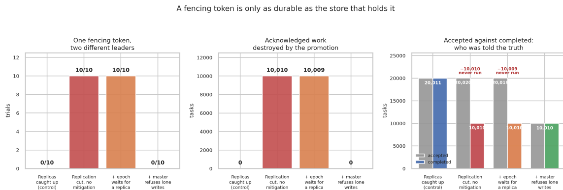
Figure 4: What a Redis failover does to the fence
