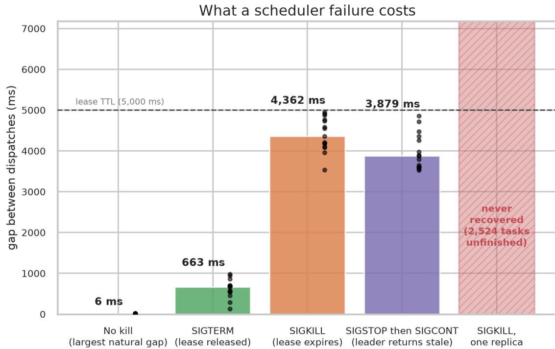
Figure 1: Failover outage by arm
