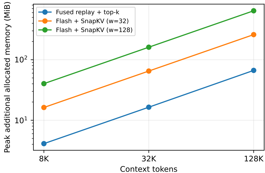
A10G, BF16, B=1, Hq=4, Hkv=2, D=64; single layer, 10% retention
