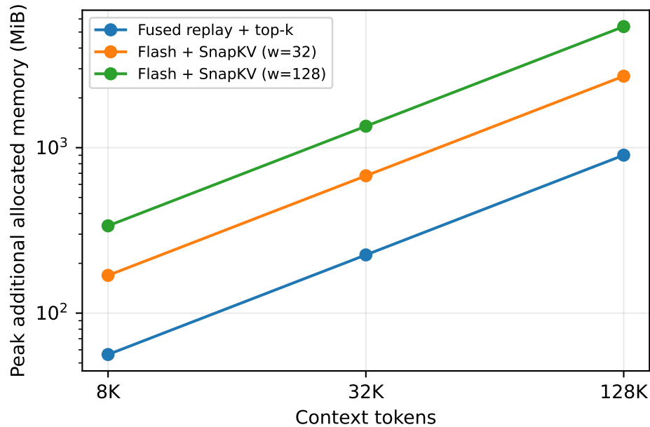
A10G, BF16, B=1, Hq=28, Hkv=4, D=128; single layer, 10% retention
