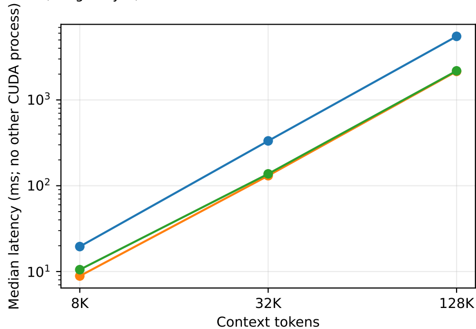
A10G, BF16, B=1, Hq=28, Hkv=4, D=128; single layer, 10% retention
