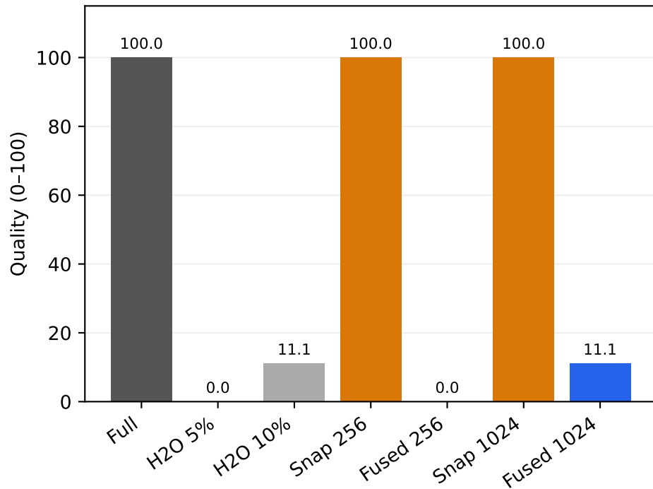
Needle: 9 prompts
