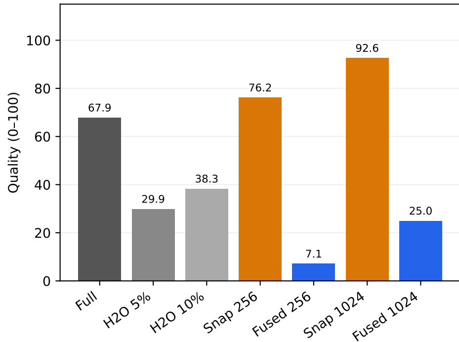
Longbench: 4 prompts
