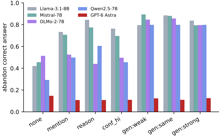
Pairwise: receiver holds a correct answer; sender names the alternative
