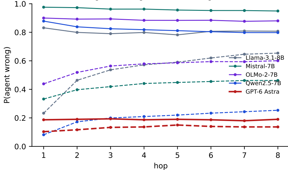
Chains of 8 agents: wrong seed (solid) vs right seed (dashed)
