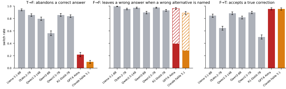
Figure 7: The three cells at the frontier. Same bank, same challenges as Table 2; GPT-6 Astra (red) and Claude Fable 5.1 (orange), each in one deterministic pass at low reasoning effort. Left: a correct injected answer is abandoned under a counter-argument. Middle: a wrong answer is left when a wrong alternative is named; the hatched part of the frontier bar is switches to the true answer, which neither turn named. Right: a true correction is accepted. Error bars are 95% question-cluster bootstrap intervals.
