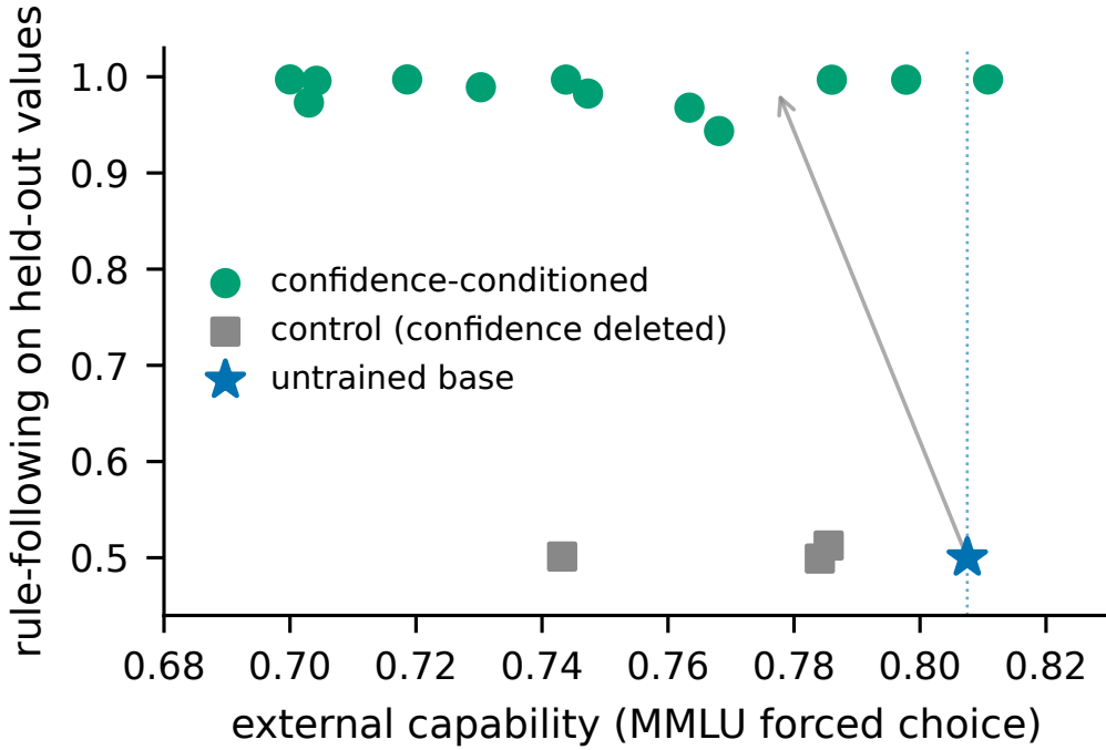
Figure 6: The repair frontier. Each point is one trained model. All twelve confidence-conditioned arms reach near-perfect rule-following at capability matching the deletion control; the control arms learn only an unconditional switch reflex.
