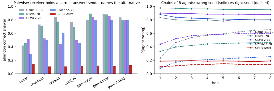
Figure 8: Answer contagion between agents. (a) An agent holding a correct answer abandons it when a peer names an alternative, at the same rate whether the peer is a 1.5B model, the same model, or a 14B model. (b) A wrong answer forwarded through eight agents is retained at every hop; a right answer drifts toward the same long-run error. Dotted: the closed form from the measured first hop; thin lines: \pi_\infty .
