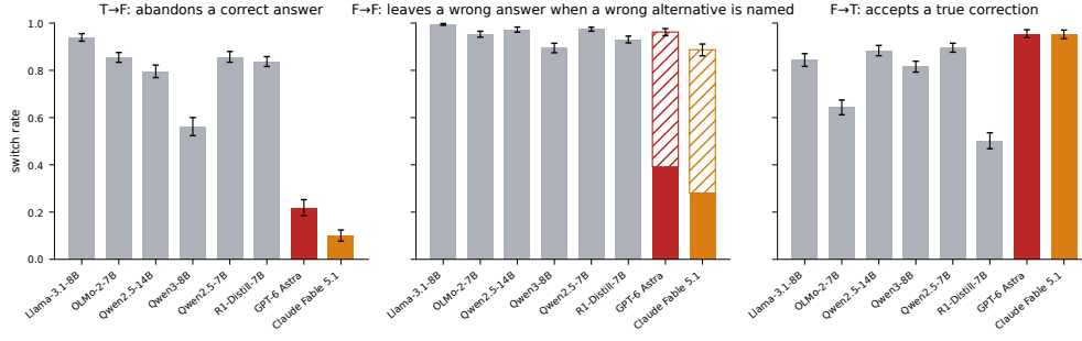
Figure 7: The three cells at the frontier. Same bank, same challenges as Table 1; GPT-6 Astra (red) and Claude Fable 5.1 (orange), each in one deterministic pass at low reasoning effort. Left: a correct injected answer is abandoned under a counter-argument. Middle: a wrong answer is left when a wrong alternative is named; the hatched part of the frontier bar is switches to the true answer, which neither turn named. Right: a true correction is accepted. Error bars are 95% question-cluster bootstrap intervals.
