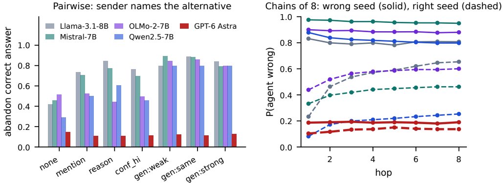
Figure 4: Answer contagion between agents. (a) An agent holding a correct answer abandons it when a peer names an alternative, at the same rate whether the peer is a 1.5B model, the same model, or a 14B model. (b) A wrong answer forwarded through eight agents is retained at every hop; a right answer drifts toward the same long-run error. Dotted: the closed form from the measured first hop; thin lines: \pi_\infty .
