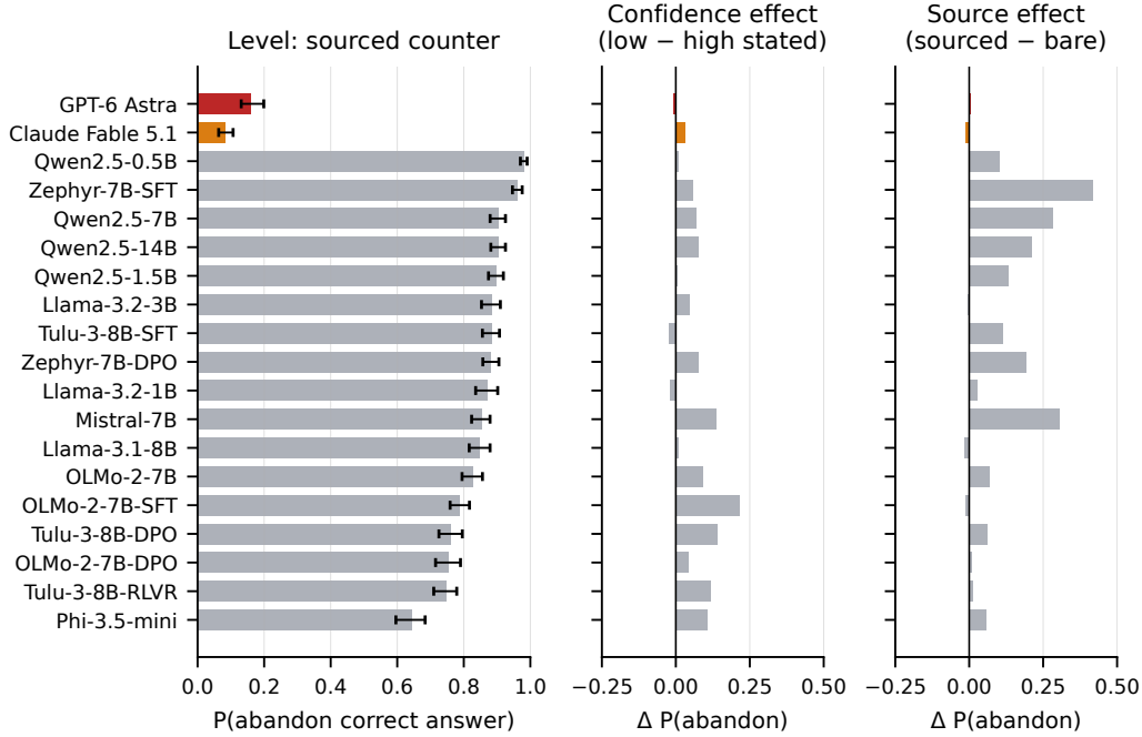
Figure 3: The level collapses, the structure survives. Seventeen open checkpoints, GPT-6 Astra (red) and Claude Fable 5.1 (orange) on the decomposition protocol of Appendix A, correct self-authored claims under a sourced counter-argument. Left: abandonment, sorted. Middle: what stated confidence adds (abandonment at low minus high stated confidence). Right: what the source adds (sourced minus bare counter-argument). The frontier models abandon a fifth (Astra) and a tenth (Fable) as often as a 7B model and use their confidence and the source exactly as little.
