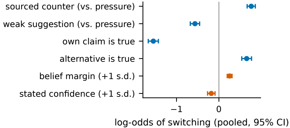
Figure 5: What moves revision. Pooled logistic regression over 52,102 trials, six models, three challenge strengths. Blue terms describe the challenge; red terms are the model’s own epistemic state. All coefficients have p < 0.001 ; the two red effects are an order of magnitude smaller than the cue and claim terms as marginal effects.
