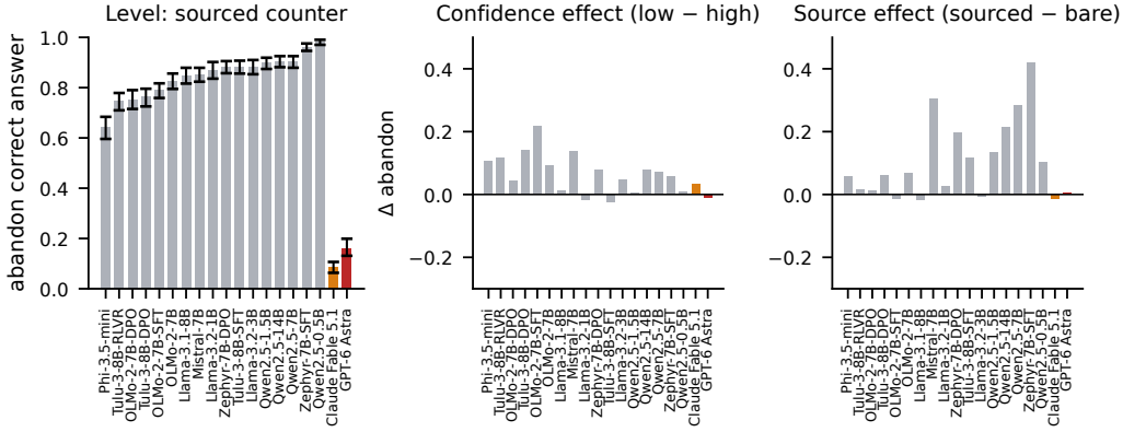
Figure 3: The level collapses, the structure survives. Seventeen open checkpoints, GPT-6 Astra (red) and Claude Fable 5.1 (orange) on the decomposition protocol of Appendix A, correct self-authored claims under a sourced counter-argument. Left: abandonment, sorted. Middle: what stated confidence adds (abandonment at low minus high stated confidence). Right: what the source adds (sourced minus bare counter-argument). The frontier models abandon a fifth (Astra) and a tenth (Fable) as often as a 7B model and use their confidence and the source exactly as little.
