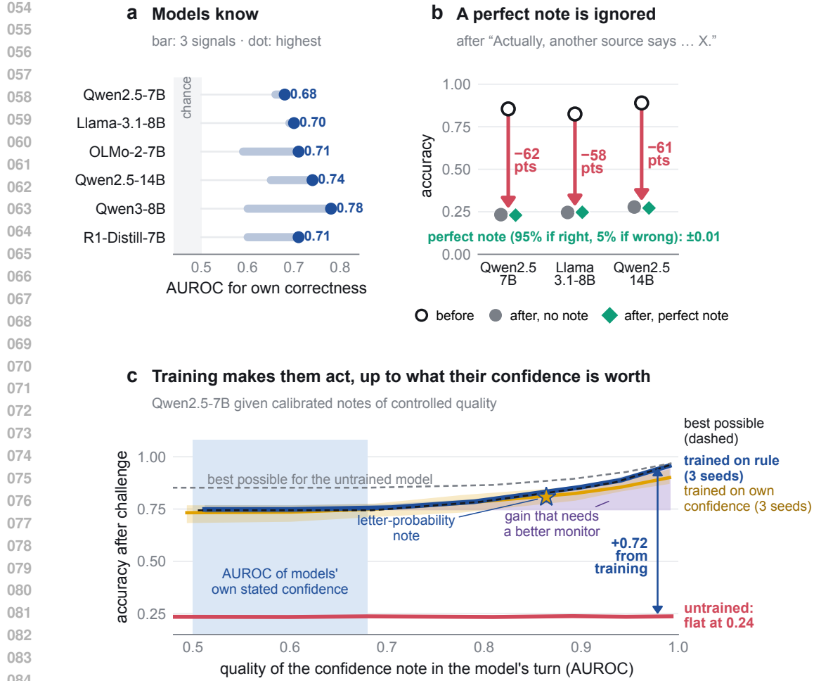
Figure 1: Models know when they might be wrong, do not act on it under a strong challenge, and can be trained to act on it, up to the quality of their confidence. (a) AUROC for the model’s own correctness on the hard bank; bars span three signals (stated confidence, P(\text{True}) , belief), dots mark the highest. (b) Accuracy before a strong challenge (open circles) and after it (red arrows: drop in points), with no note (grey) or with a perfect confidence note in the model’s own turn (green; 95% if right, 5% if wrong). The note changes post-challenge accuracy by at most 0.01. (c) Qwen2.5-7B accuracy after a strong challenge against the AUROC of a calibrated confidence note: untrained (red), rule-trained (blue), and own-confidence arm (gold); trained curves are means of three seeds with the range shaded. Two dashed curves show the best possible accuracy (keep the answer if and only if the note is at least 50%): for the untrained model (grey; 0.852 at AUROC 0.5 to 0.969 at 0.99) and for the rule-trained model, seed 0 (black), which starts lower. Blue region: the AUROC range of the models’ own stated confidence. Purple: accuracy above keeping every answer that only a better note can unlock. Star: rule-trained seed 0 given a letter-probability note (95% CI). The +0.72 bracket is rule-trained (mean) minus untrained accuracy at AUROC 0.99.
