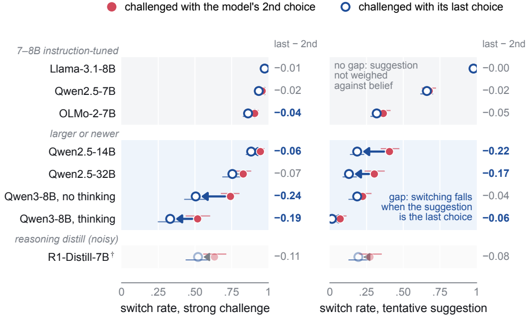
Figure 3: Qwen2.5-7B and Llama-3.1-8B switch to the answer they believe least as often as to their second choice; larger and newer models compare. Switch rate when a wrong answer is challenged with the model’s second choice (red) or last choice (open blue), under a strong challenge (left) and a tentative suggestion (right). Arrows show the change from second to last choice; thin lines are 95% CIs. Right of each panel: difference in switch rate (last minus second; bold when the 95% CI excludes zero). Items per model: 500 (7–8B), 300 (Qwen2.5-14B), 200 (Qwen2.5-32B, Qwen3-8B without thinking), 150 (thinking models). R1-Distill-7B (faded) fails the bare-doubt check, so its difference is within noise.
