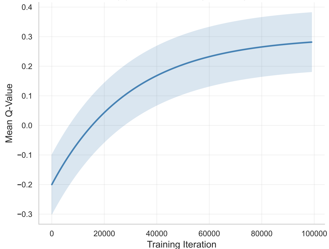
(b) Q-Value During Training
