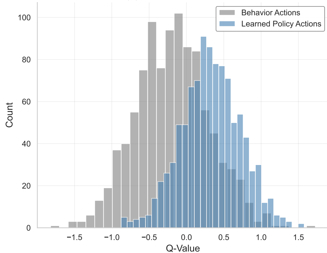
(a) Q-Value Distribution
