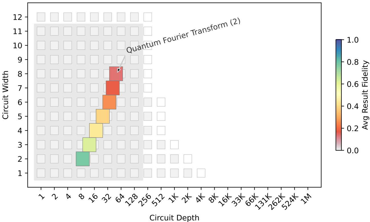
Volumetric Positioning - All Applications (Merged) Device=ibm_brisbane Jun 19, 2025 19:58:17 UTC
