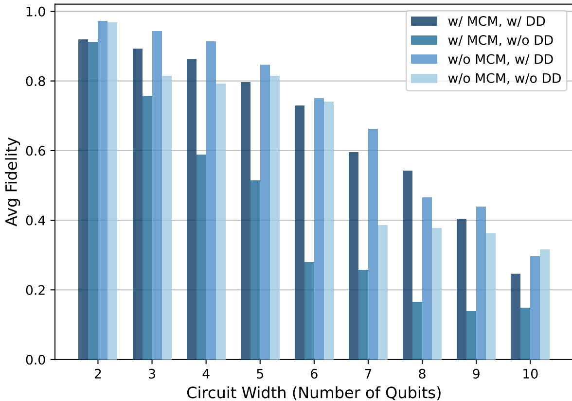
QFT method 1 Average Fidelities on IBM Pittsburgh: Four MCM/DD Variants
