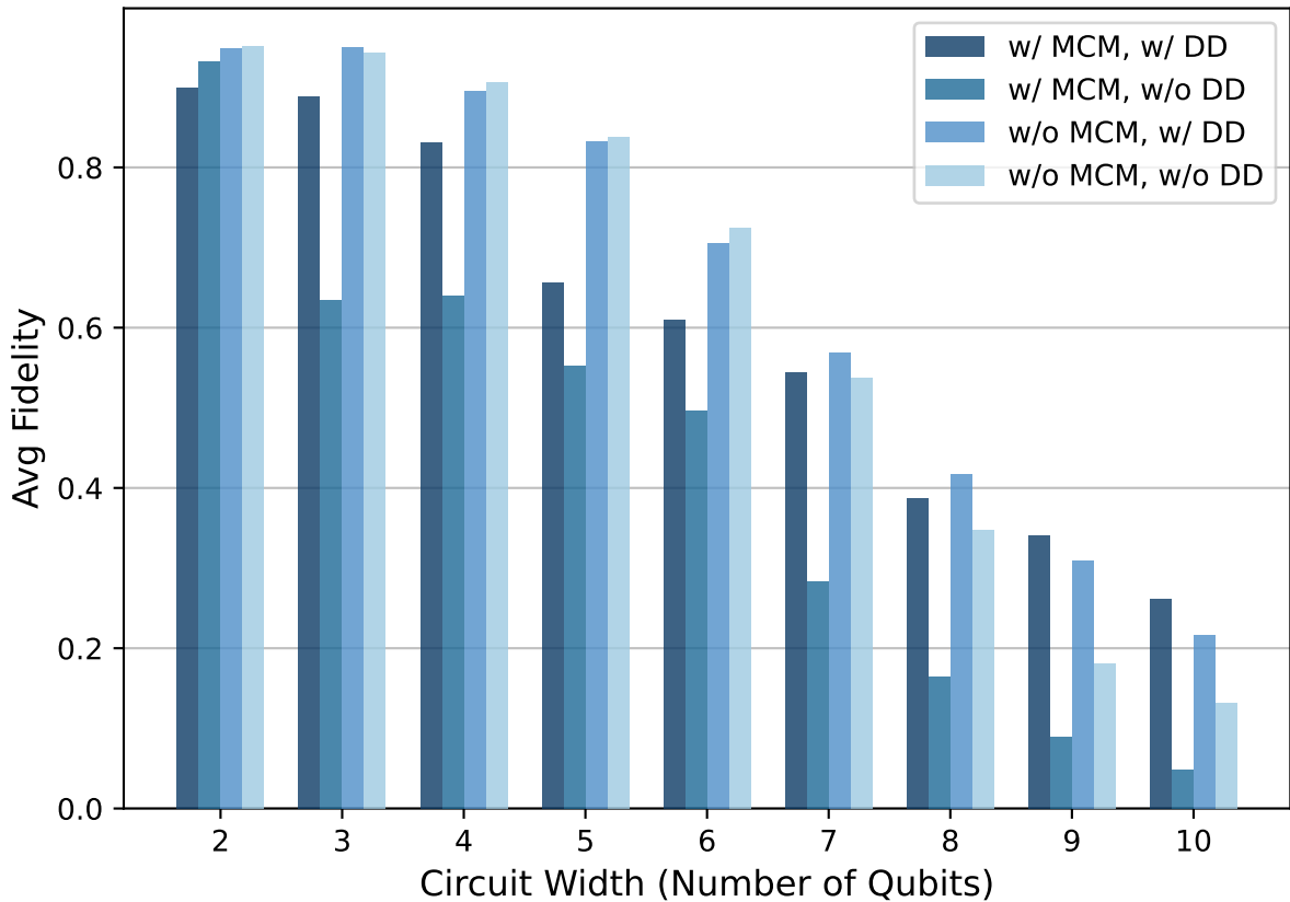
QFT Method 2 Average Fidelities on IBM Fez: Four MCM/DD Variants
