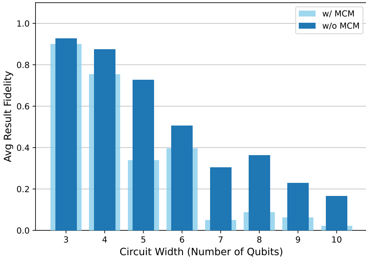
QPE comparison on IBM Fez: w/ vs w/o MCM
