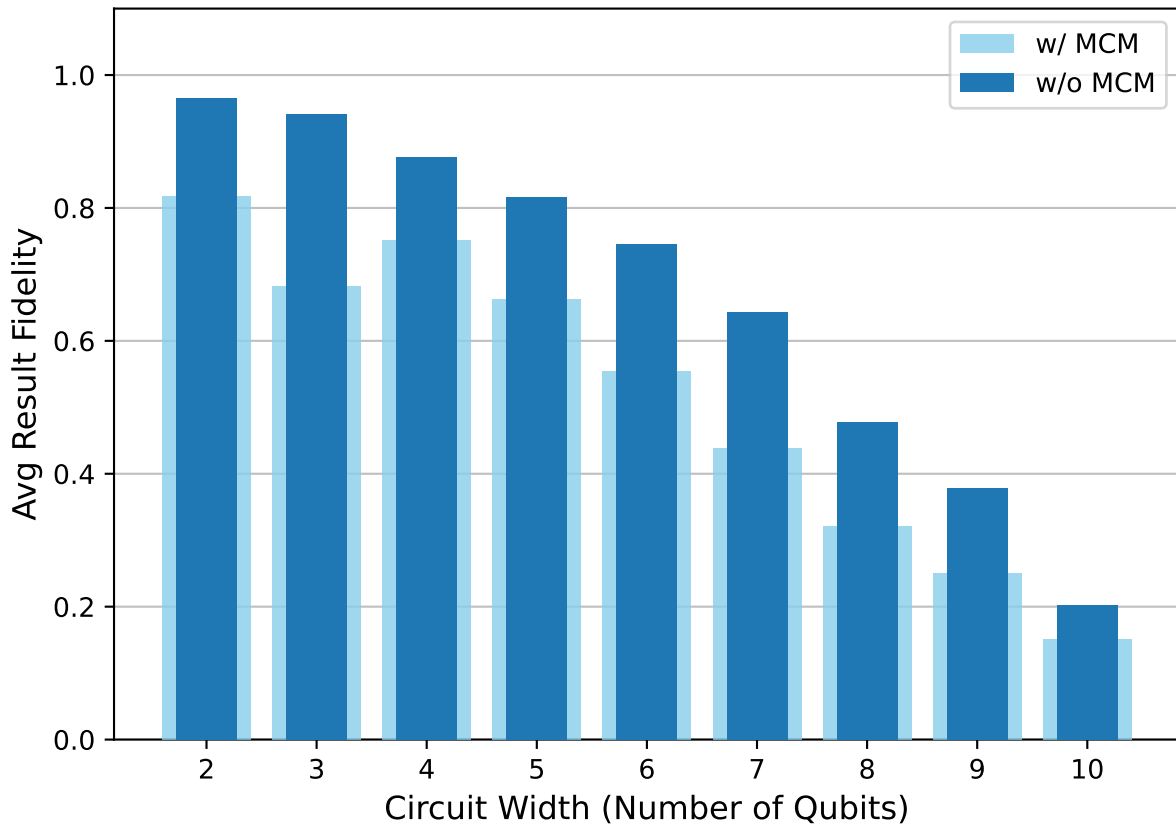
QFT method 2 comparision on IBM Fez: w/ vs w/o (MCM and DD)
