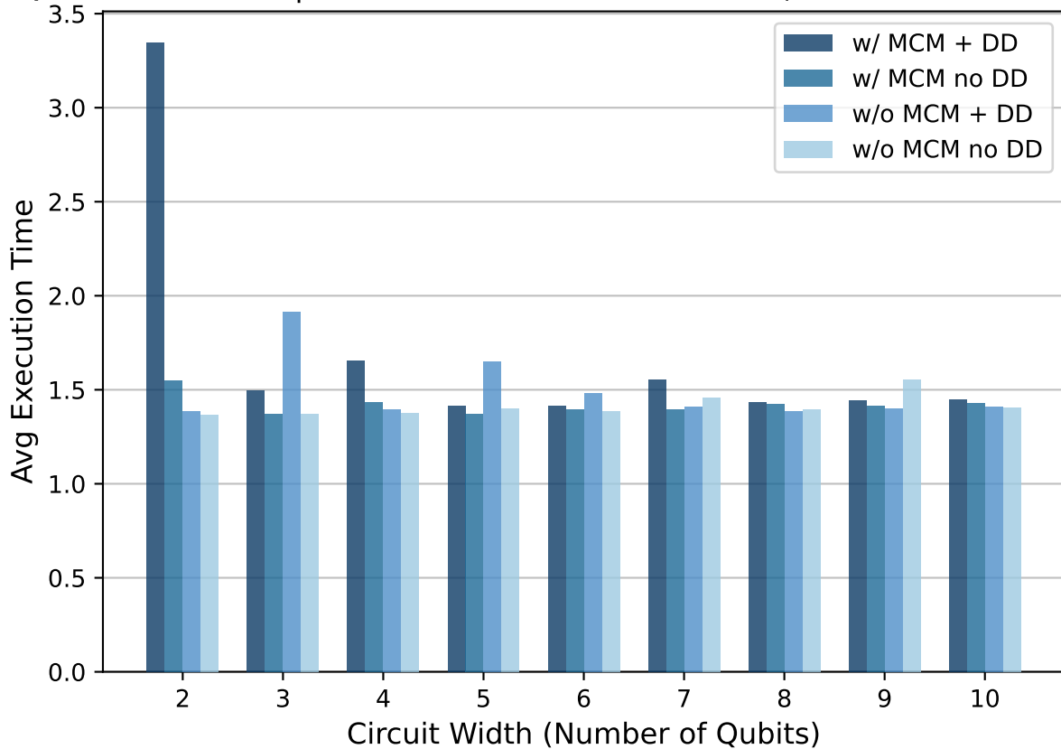
QFT method 1 comparison on IBM Fez: four variants (MCM / DD combinations)
