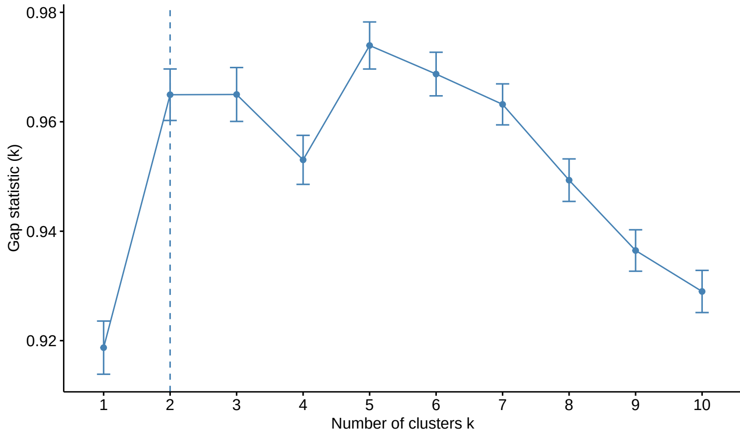
Gap statistic Tibs2001SEmax rule
